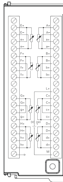
SM3TI8RTD
