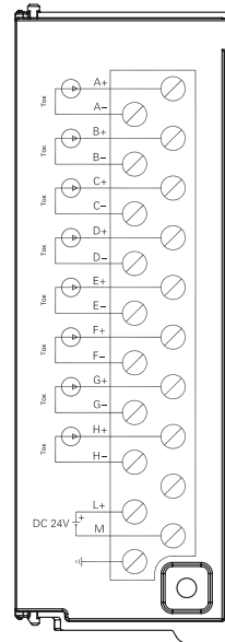
SM3A18C
