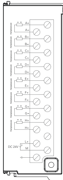
SM3A18V
