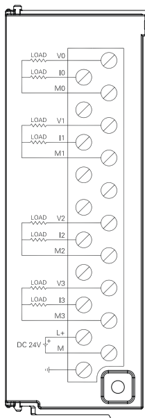
SM3AQ4
