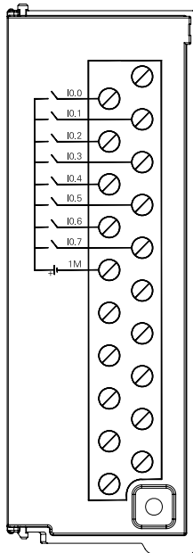
SM3DI8
