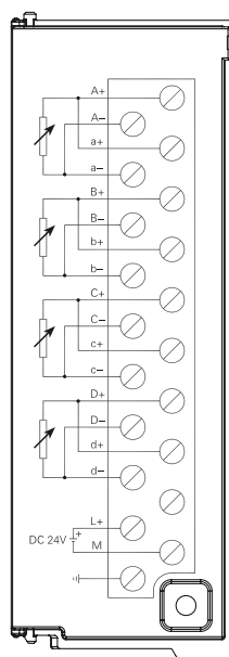
SM3TI4RTD
