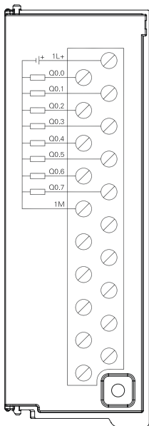
SM3DQ8T
